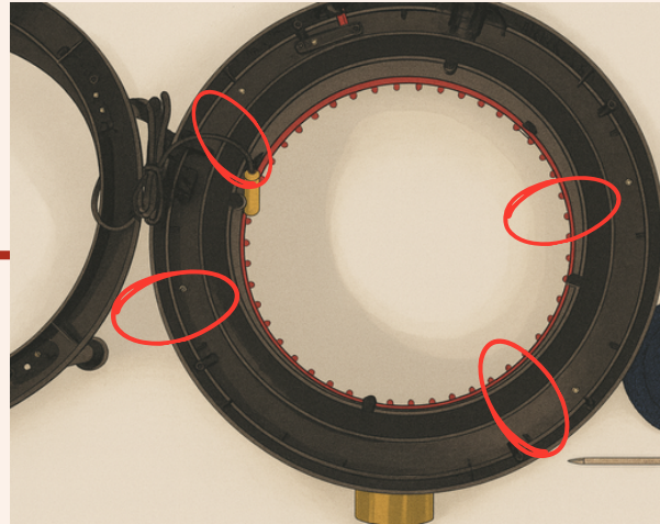
Unscrew the four screws securing the main body.
